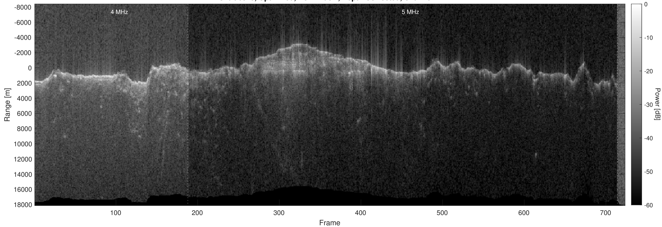
Orbit 6523, Optimized, No Window, Depth-Corrected, Channel 2
