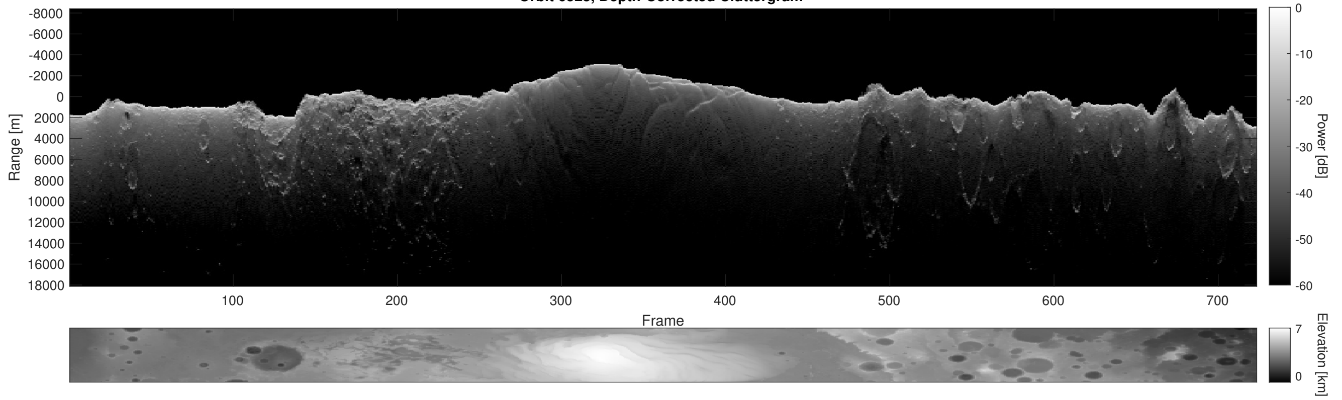
Orbit 6523, Depth-Corrected Cluttergram
