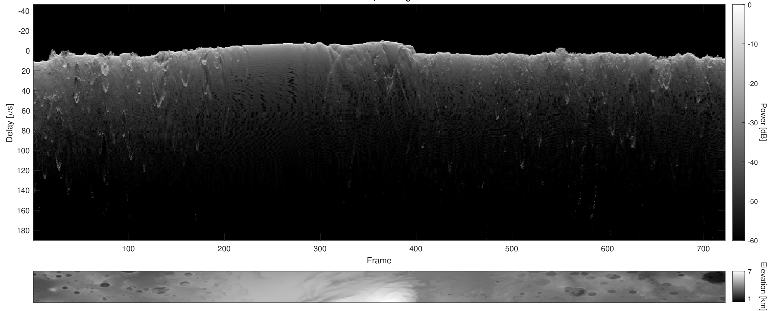
Orbit 6524, Cluttergram
