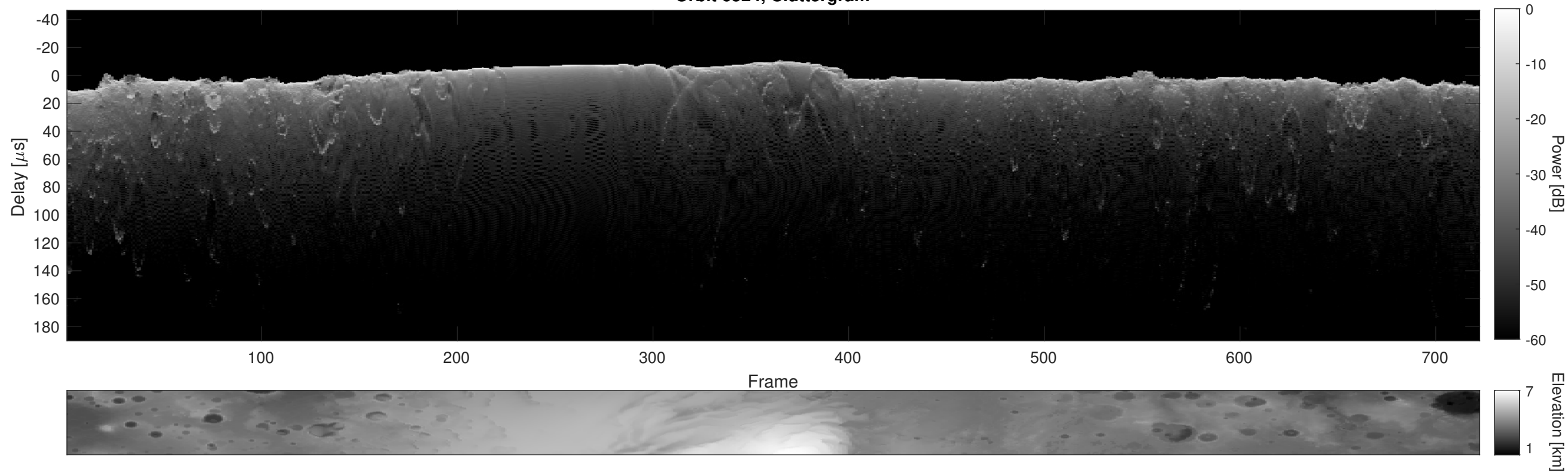
Orbit 6524, Cluttergram
