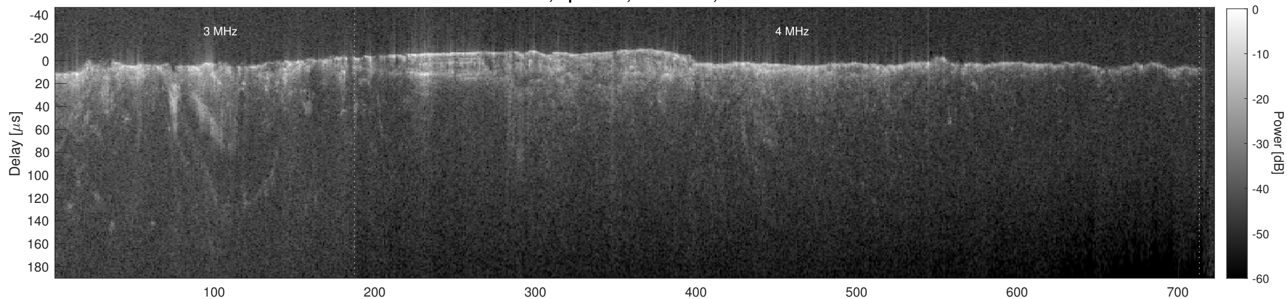
Orbit 6524, Cluttergram
