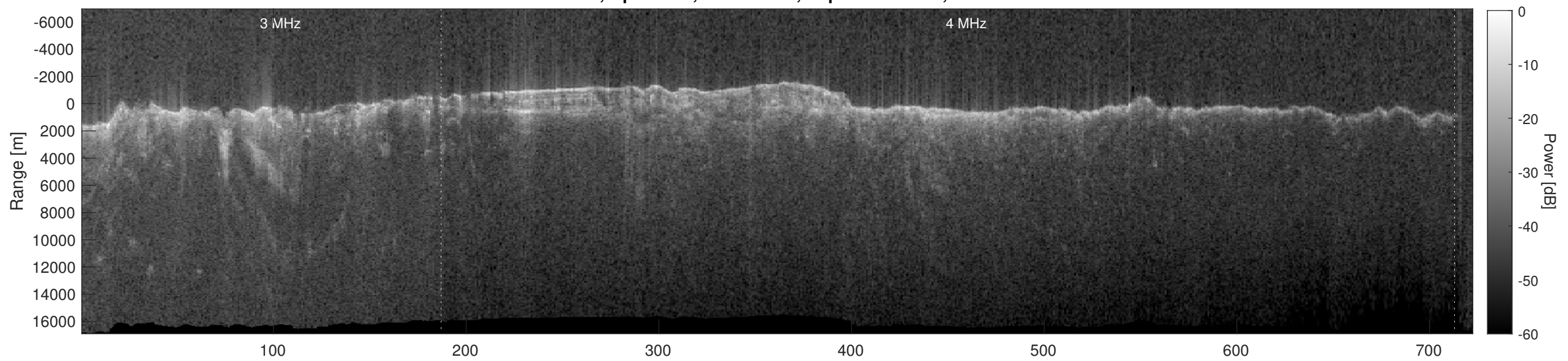
Orbit 6524, Depth-Corrected Cluttergram
