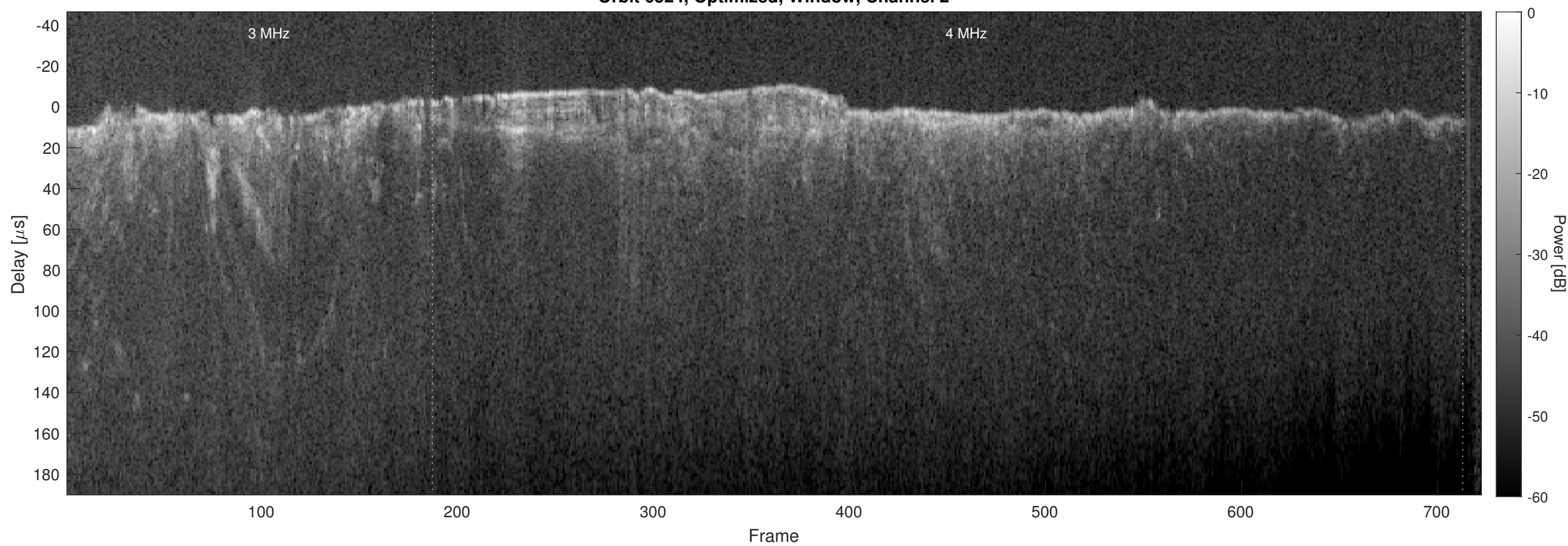
Orbit 6524, Optimized, Window, Channel 2
