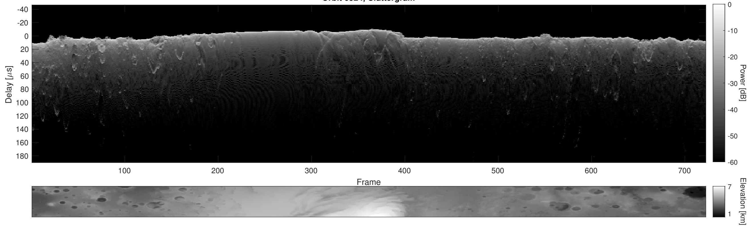
Orbit 6524, Cluttergram
