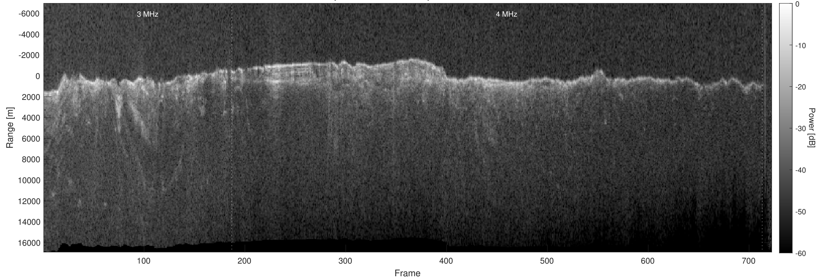
Orbit 6524, Optimized, Window, Depth-Corrected, Channel 2
