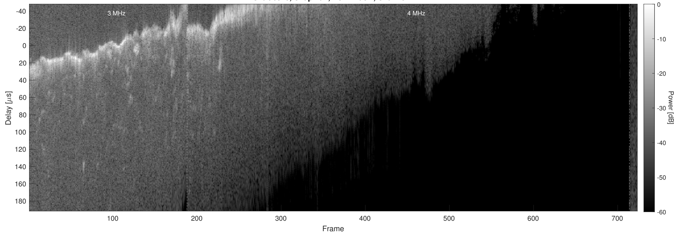
Orbit 6525, Chapman, No Window, Channel 2
