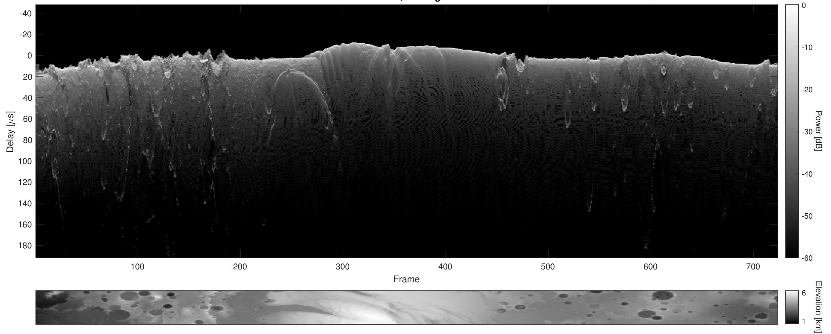
Orbit 6525, Cluttergram
