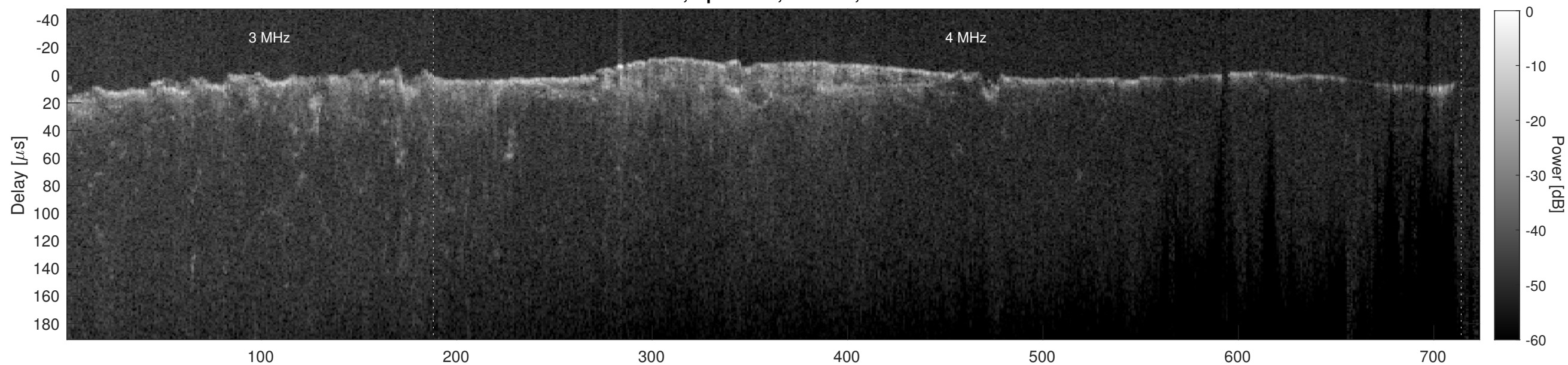
Orbit 6525, Cluttergram
