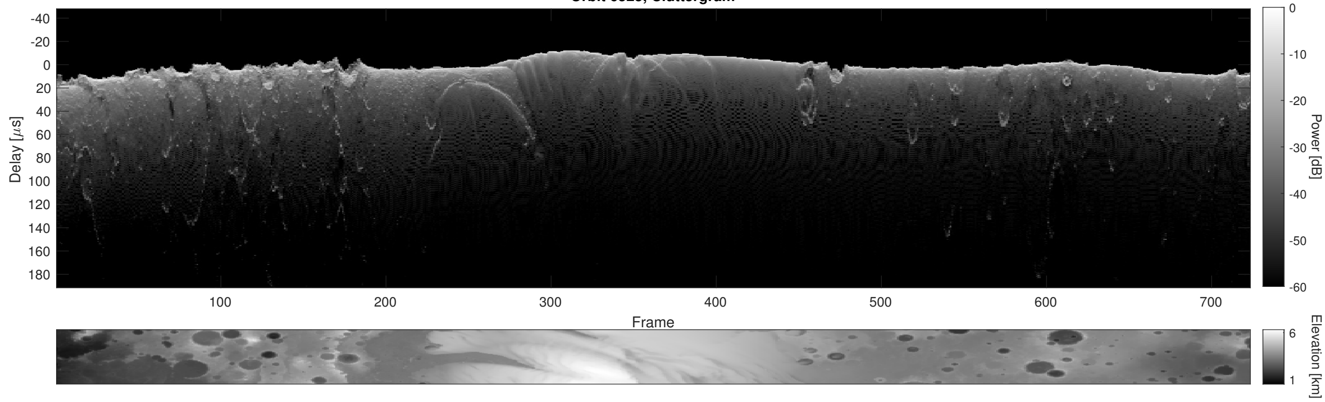
Orbit 6525, Cluttergram
