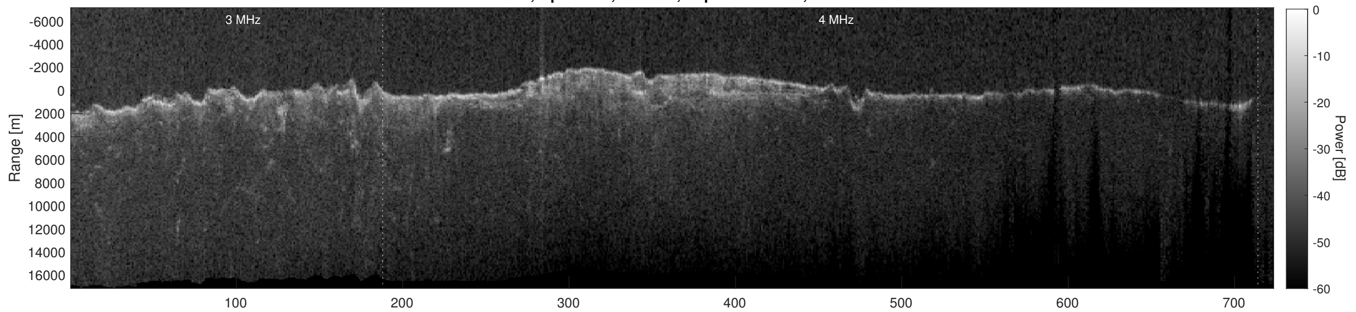
Orbit 6525, Depth-Corrected Cluttergram
