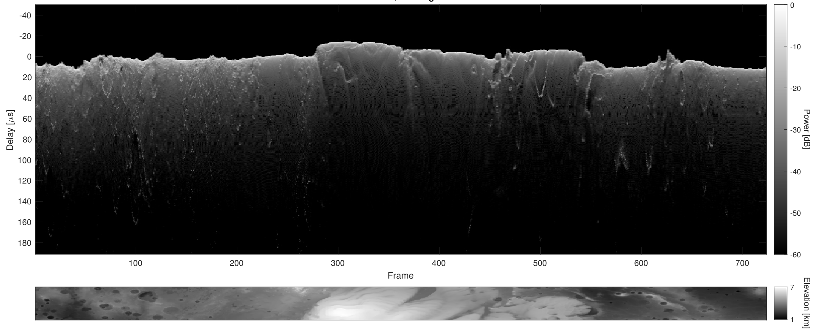
Orbit 6526, Cluttergram
