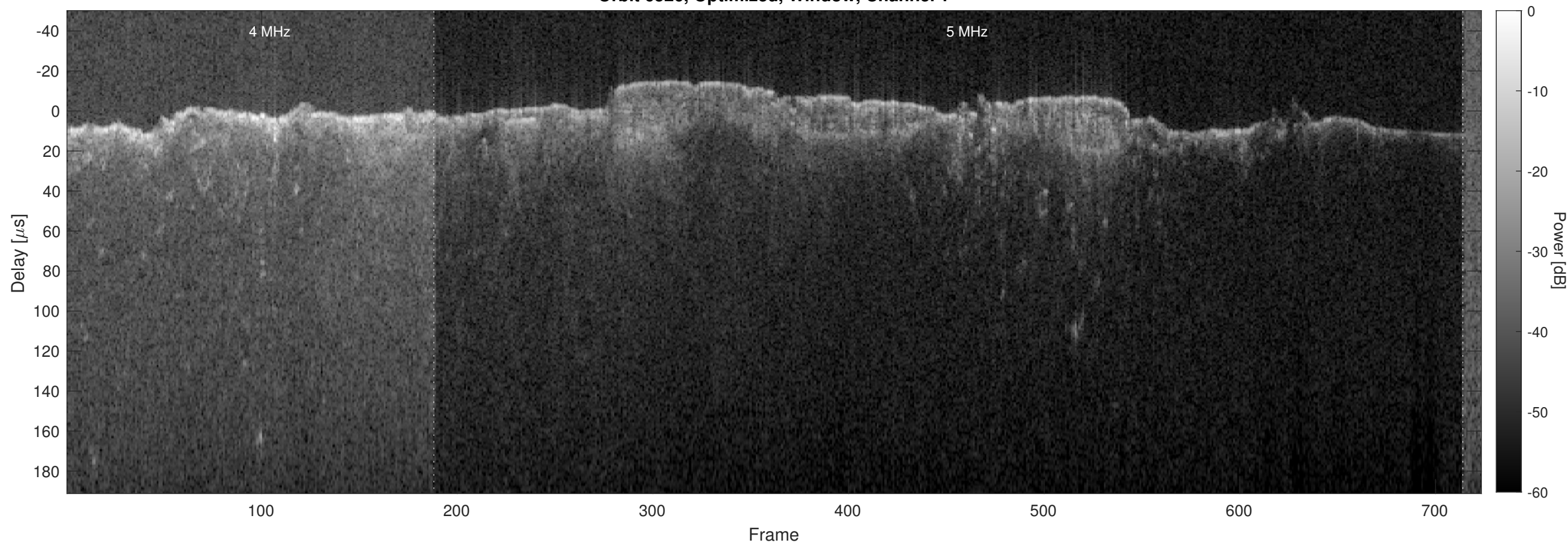
Orbit 6526, Optimized, Window, Channel 2
