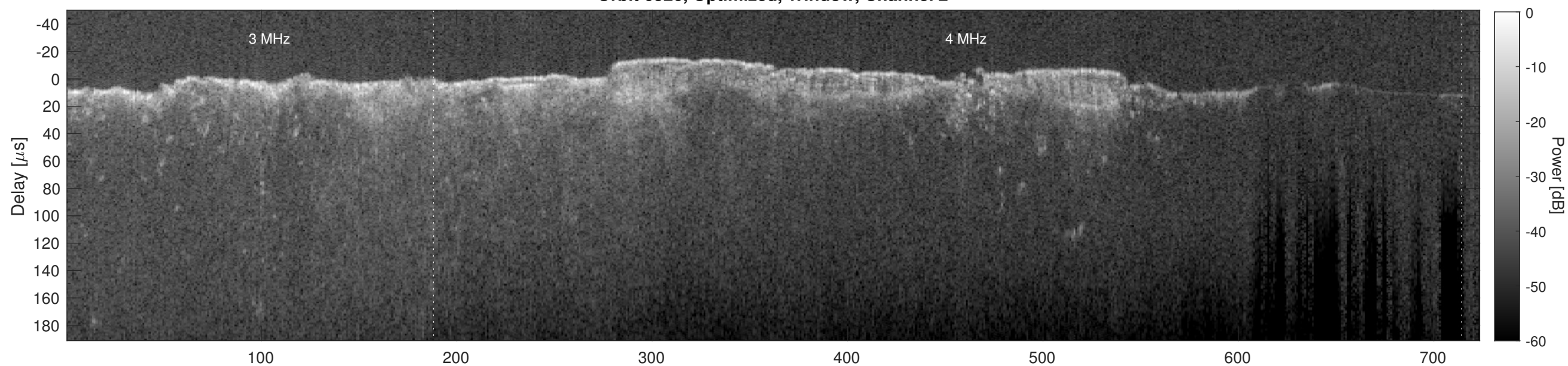
Orbit 6526, Cluttergram
