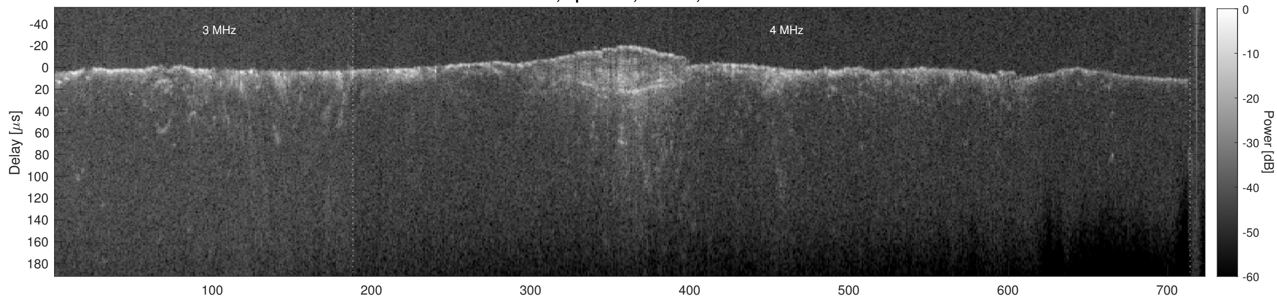
Orbit 6527, Cluttergram
