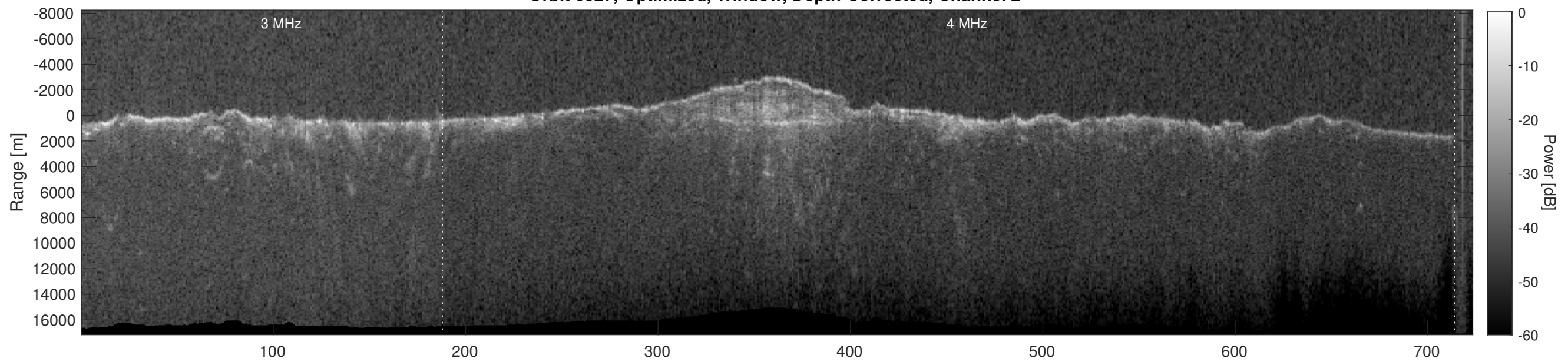
Orbit 6527, Depth-Corrected Cluttergram
