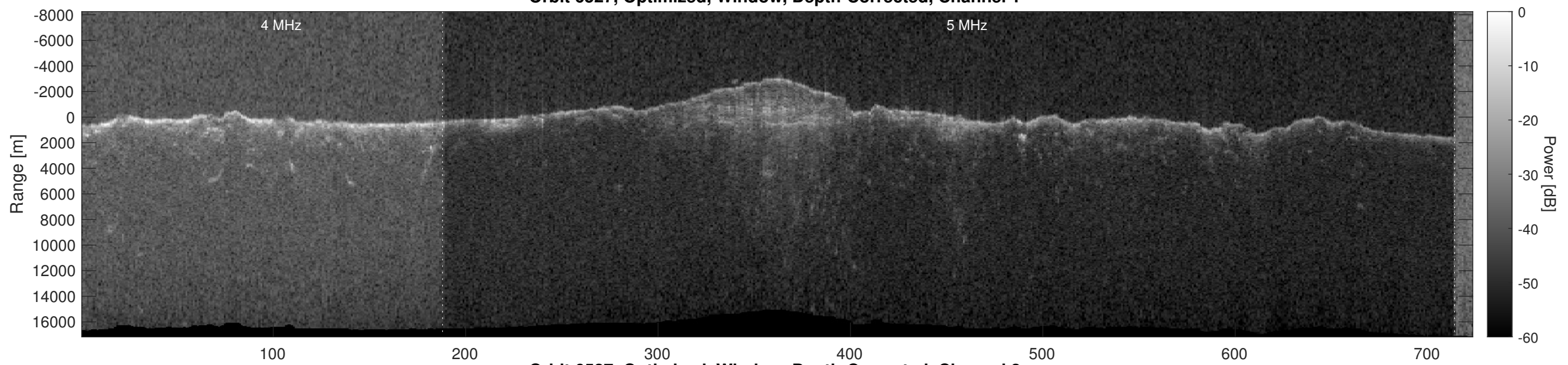
Orbit 6527, Optimized, Window, Depth-Corrected, Channel 2
