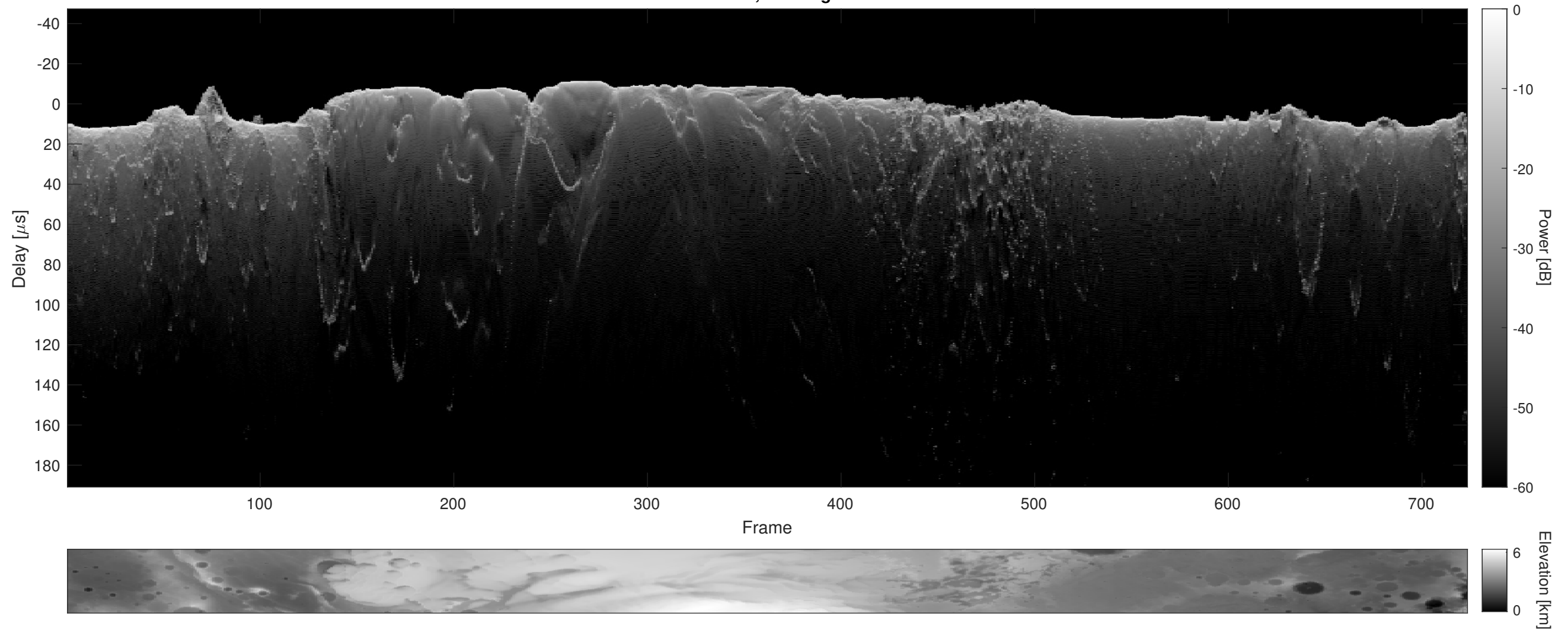
Orbit 6528, Cluttergram
