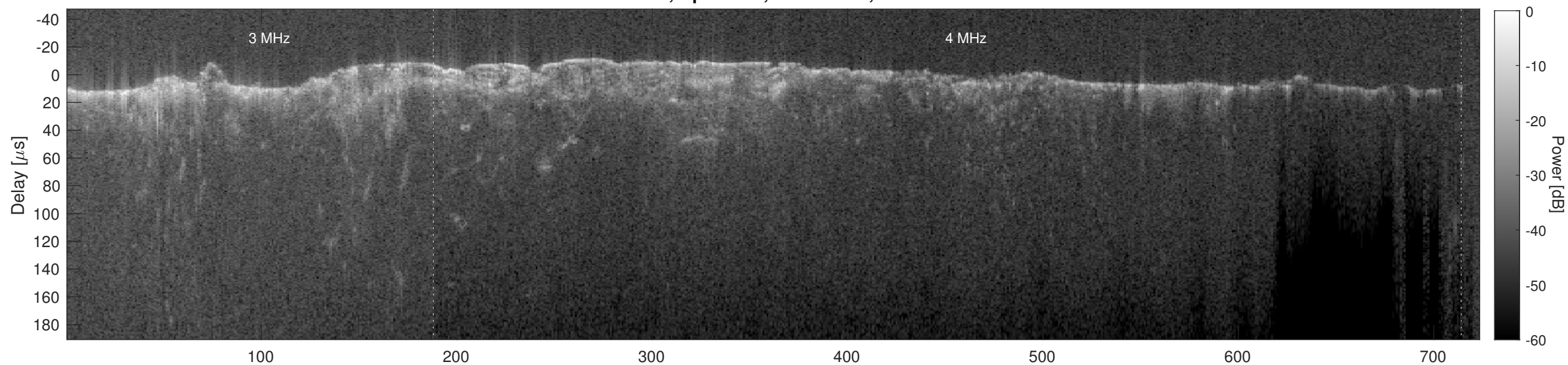
Orbit 6528, Cluttergram
