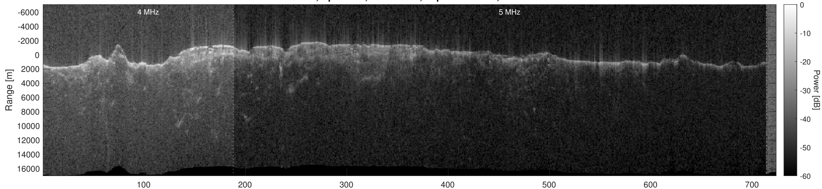
Orbit 6528, Optimized, No Window, Depth-Corrected, Channel 2
