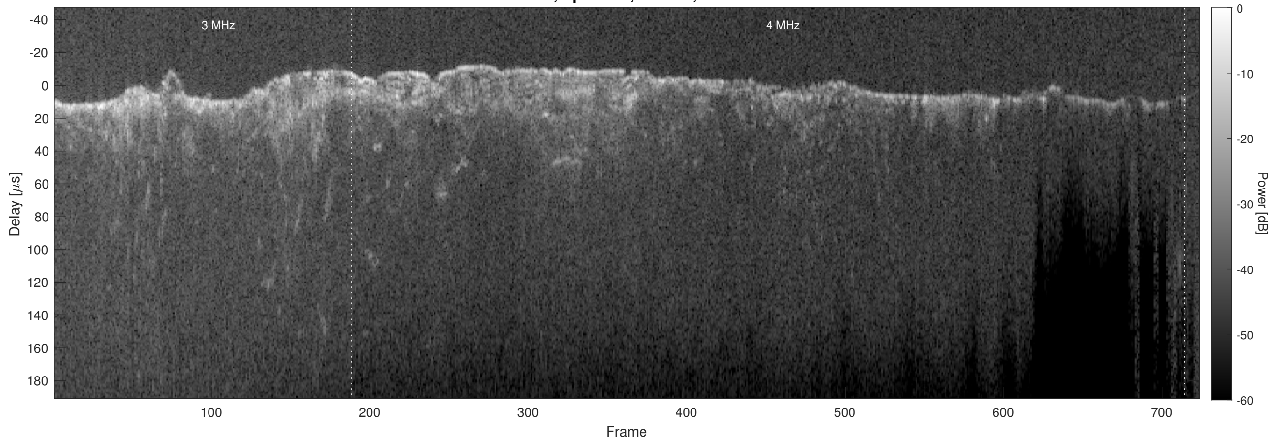
Orbit 6528, Optimized, Window, Channel 2
