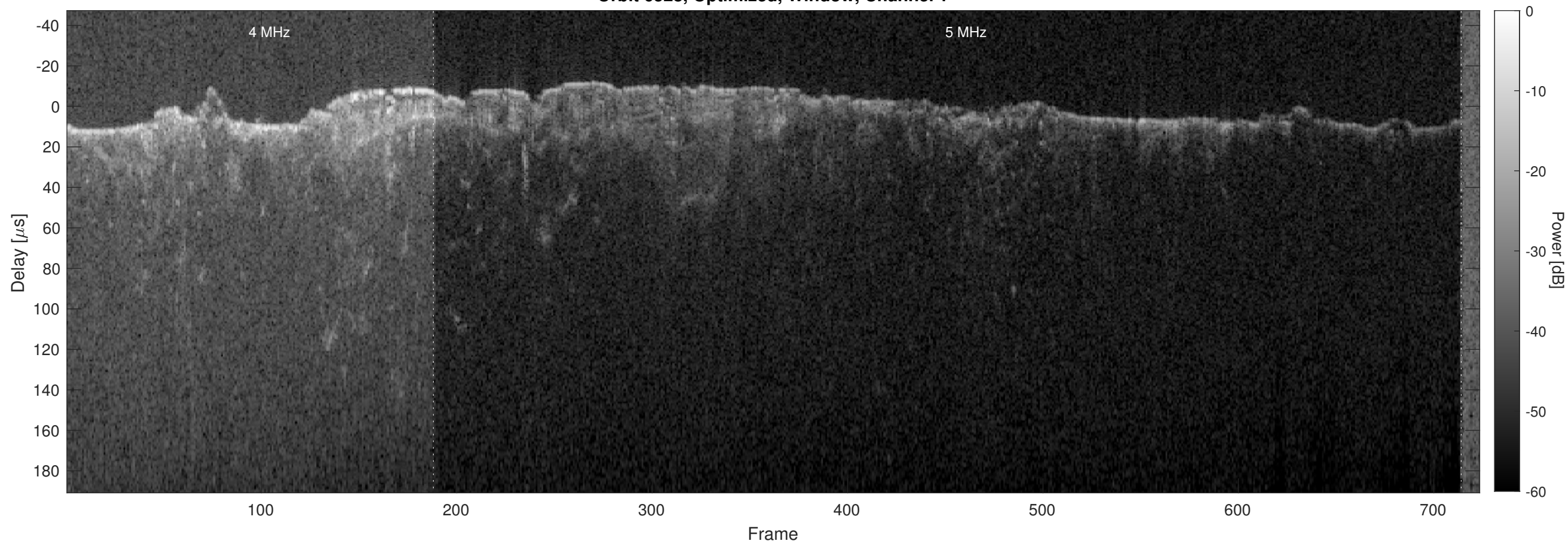
Orbit 6528, Optimized, Window, Channel 2
