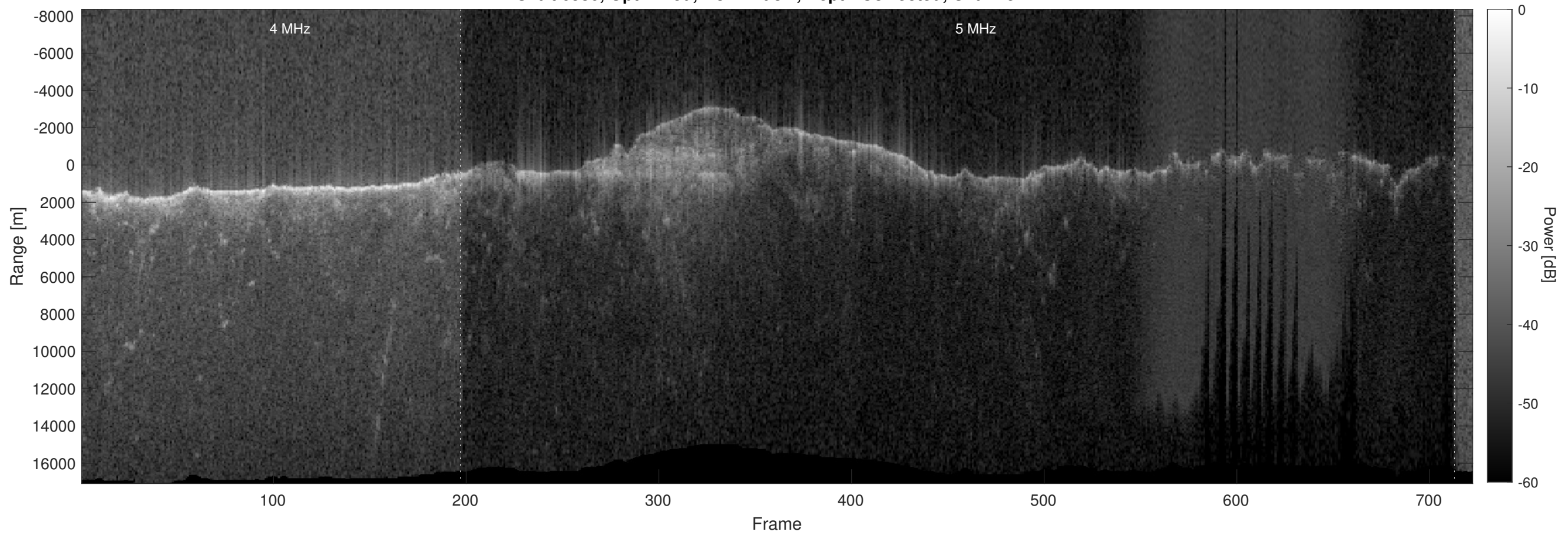
Orbit 6530, Optimized, No Window, Depth-Corrected, Channel 2
