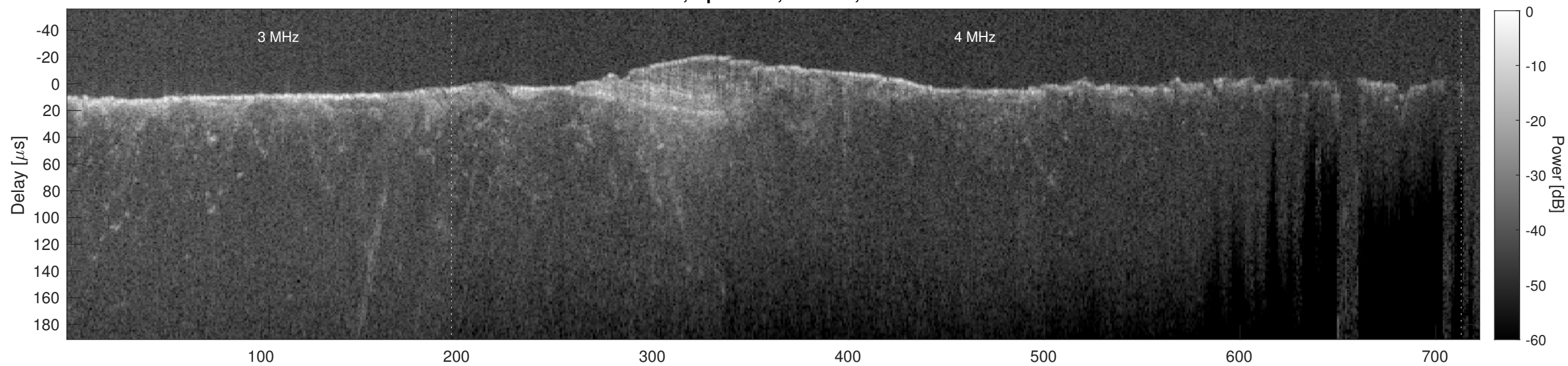
Orbit 6530, Cluttergram
