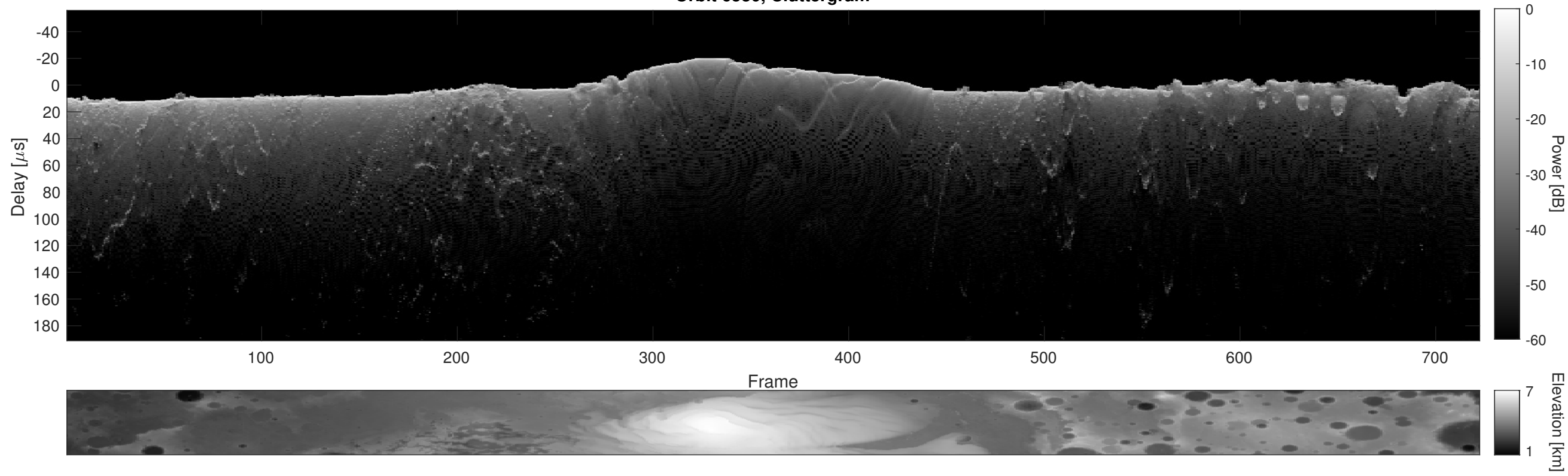
Orbit 6530, Cluttergram
