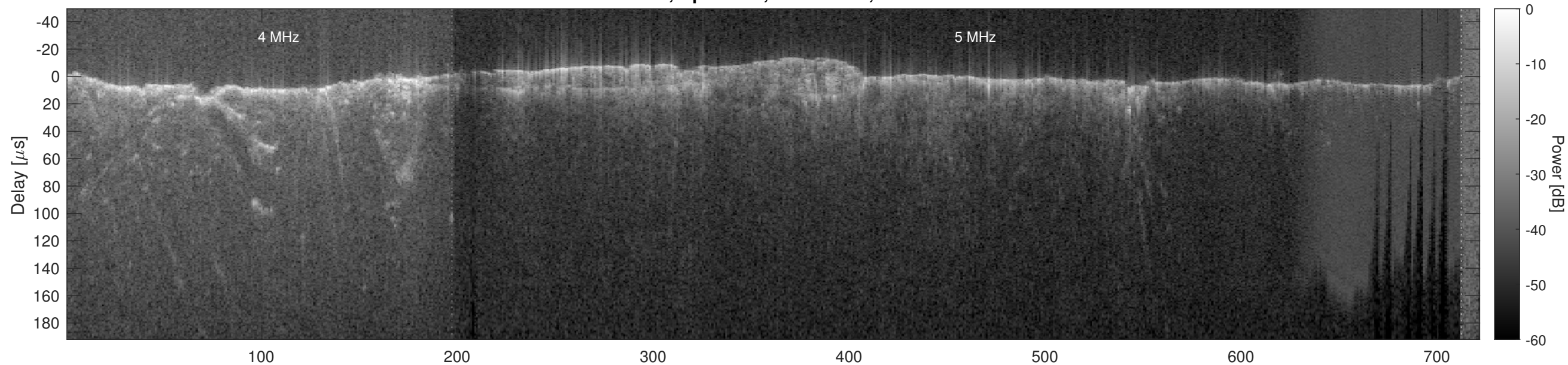
Orbit 6531, Optimized, No Window, Channel 2
