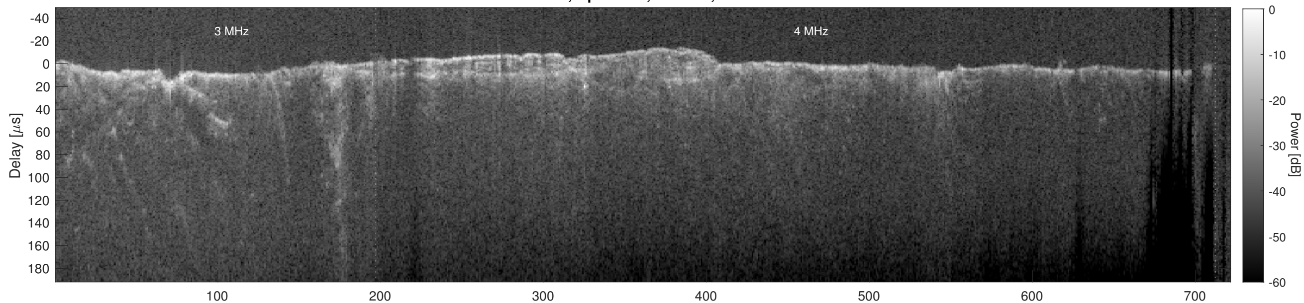
Orbit 6531, Cluttergram
