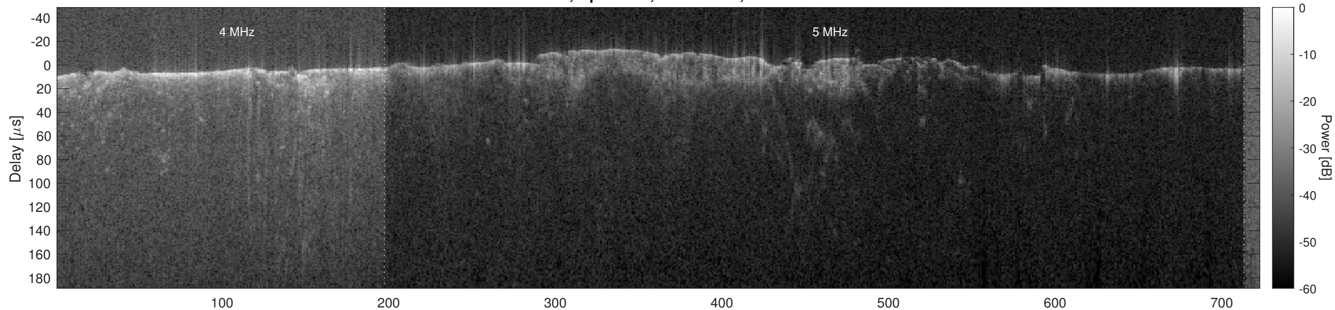
Orbit 6533, Optimized, No Window, Channel 2
