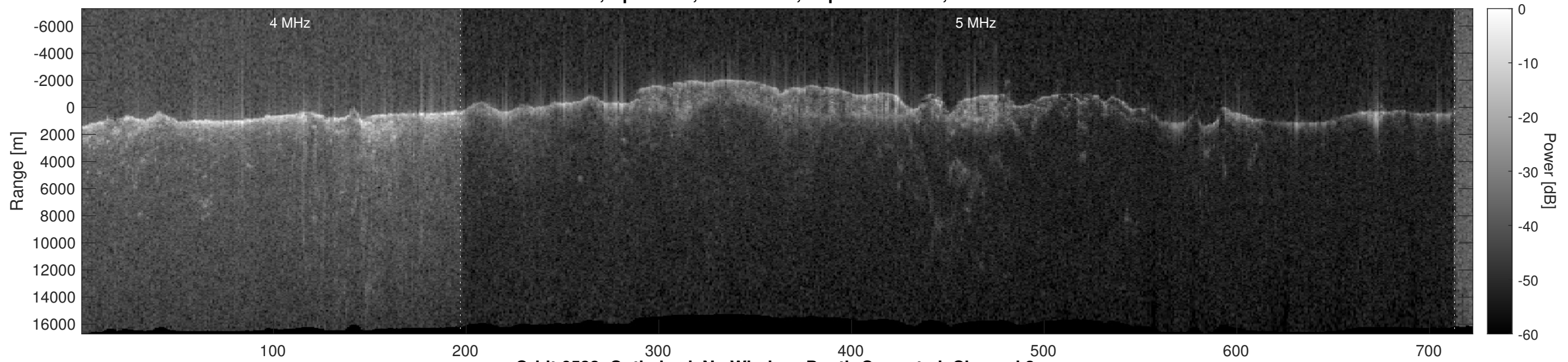
Orbit 6533, Optimized, No Window, Depth-Corrected, Channel 2
