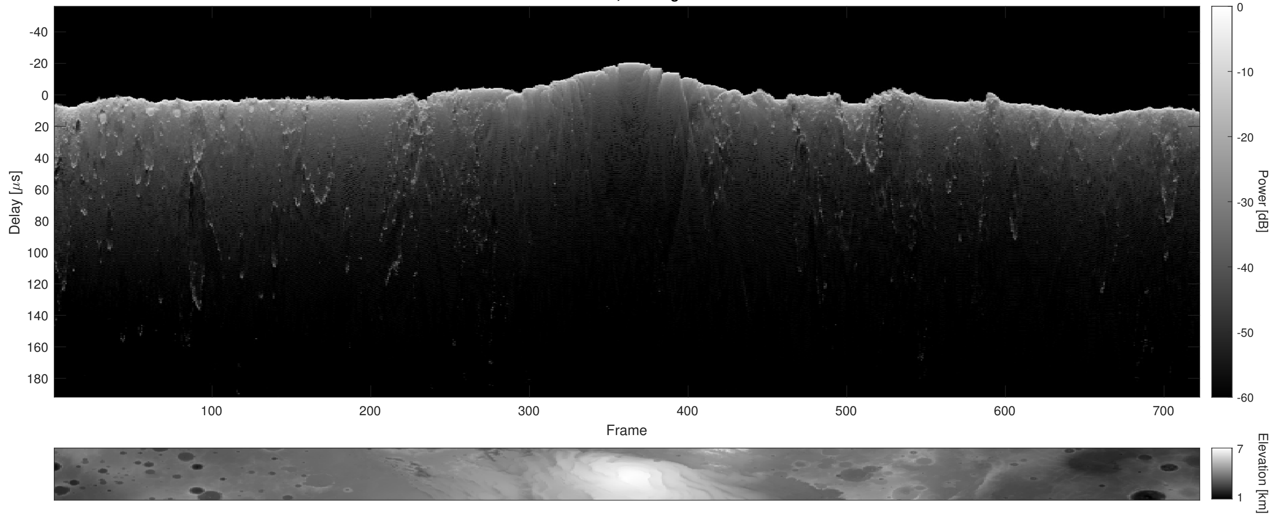
Orbit 6534, Cluttergram
