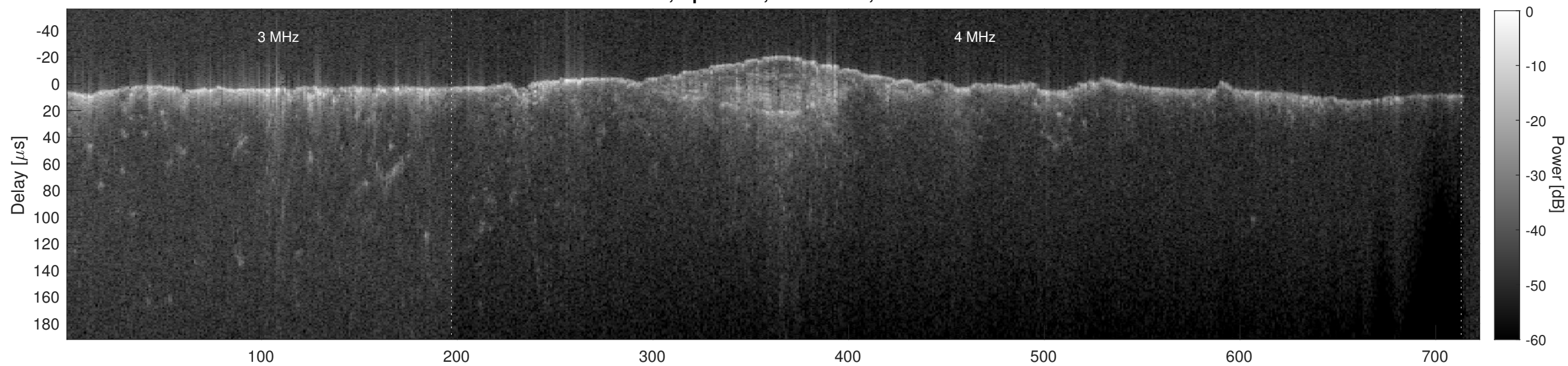
Orbit 6534, Cluttergram
