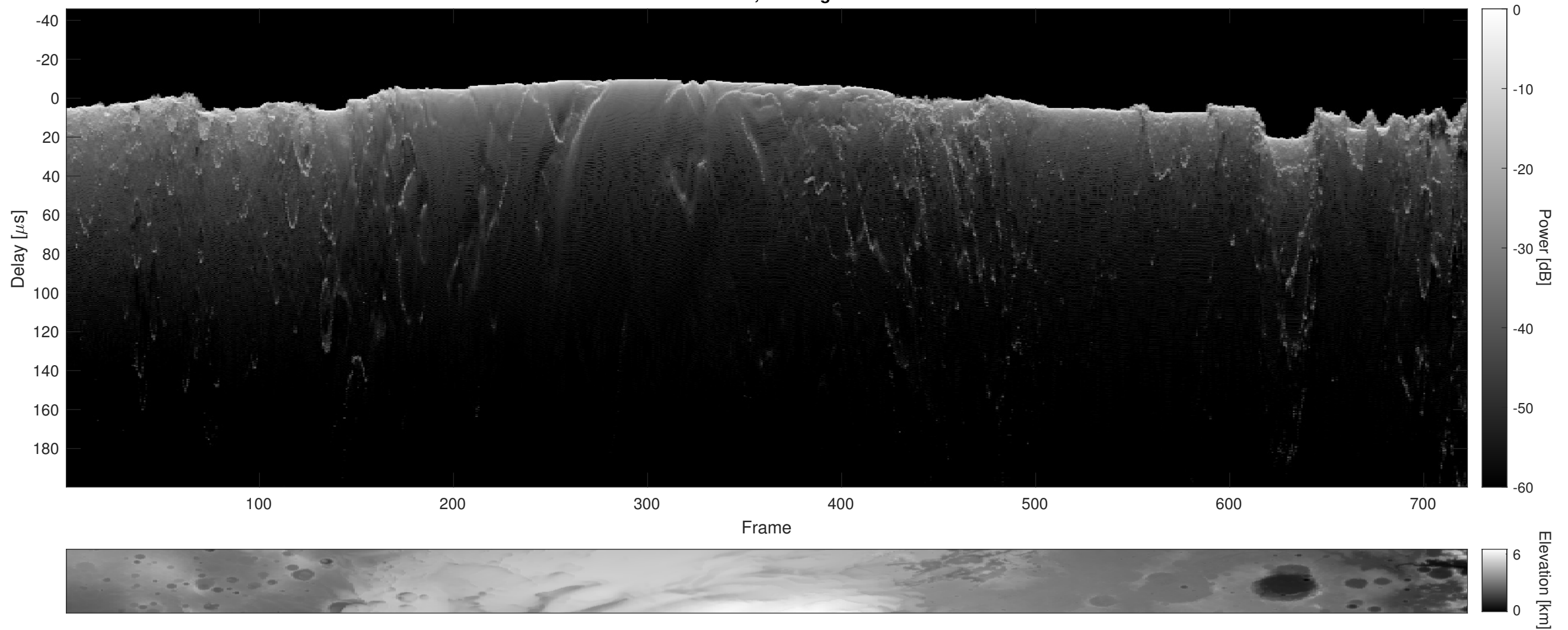
Orbit 6535, Cluttergram
