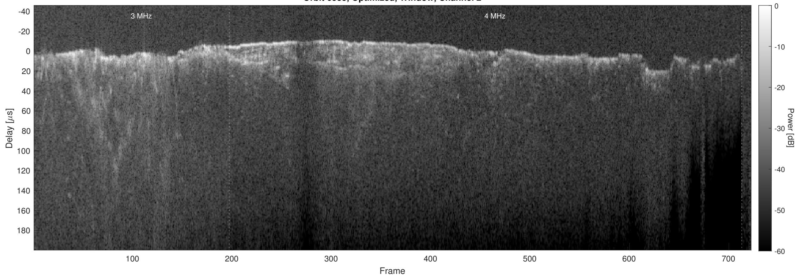
Orbit 6535, Optimized, Window, Channel 2
