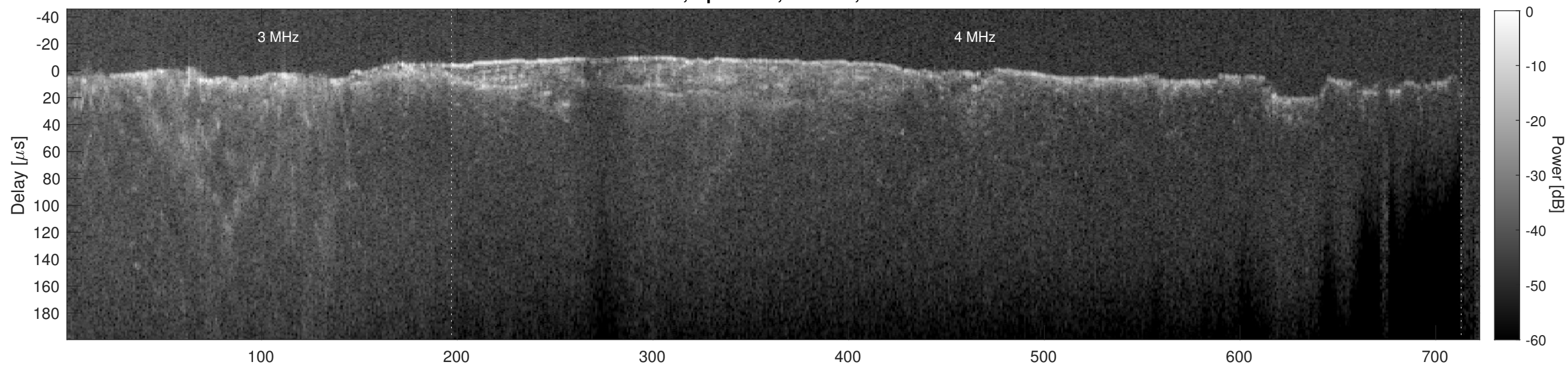
Orbit 6535, Cluttergram
