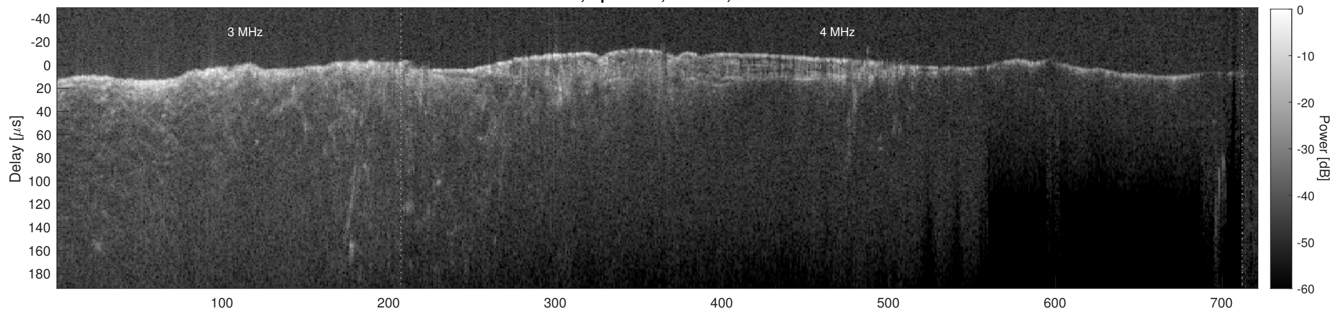
Orbit 6536, Cluttergram
