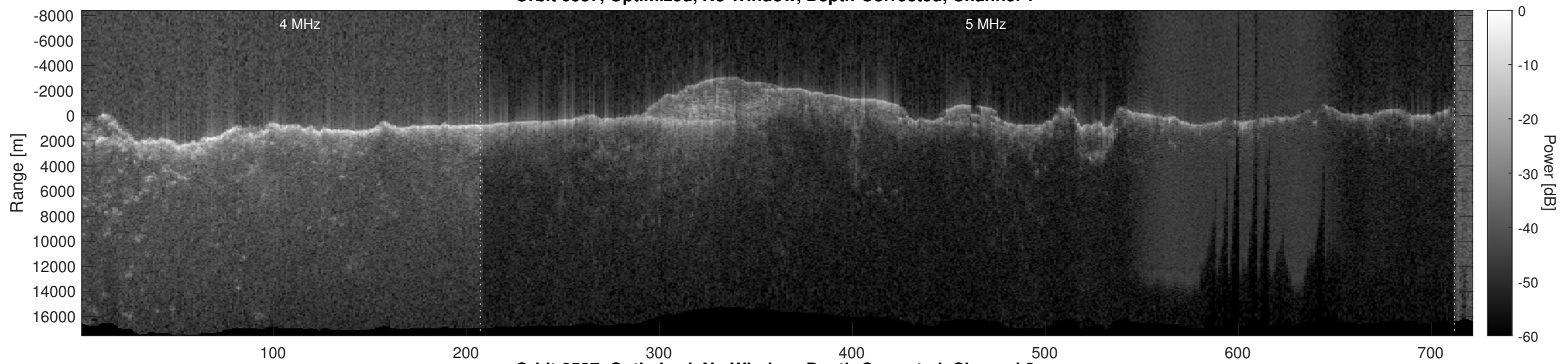
Orbit 6537, Optimized, No Window, Depth-Corrected, Channel 2
