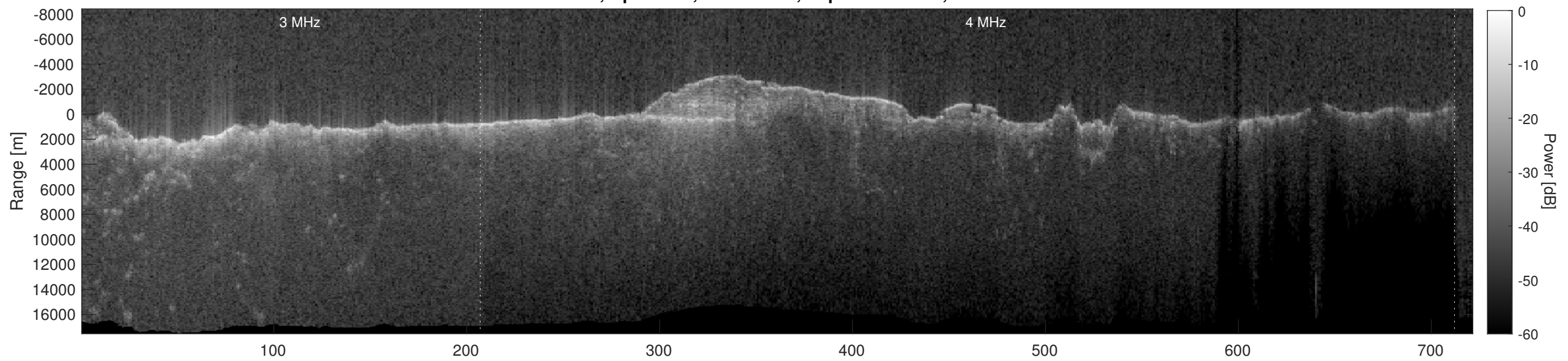
Orbit 6537, Depth-Corrected Cluttergram
