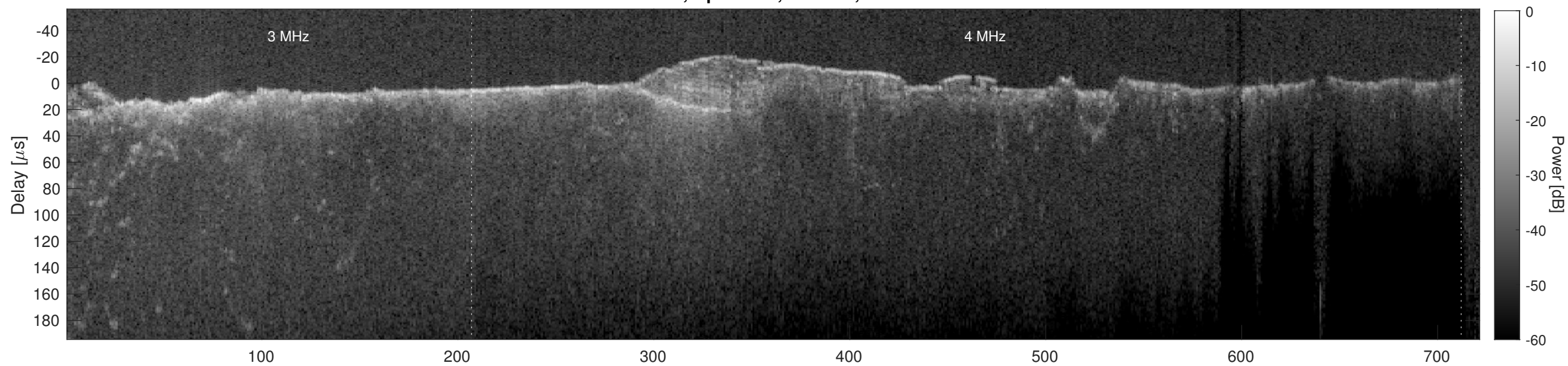
Orbit 6537, Cluttergram
