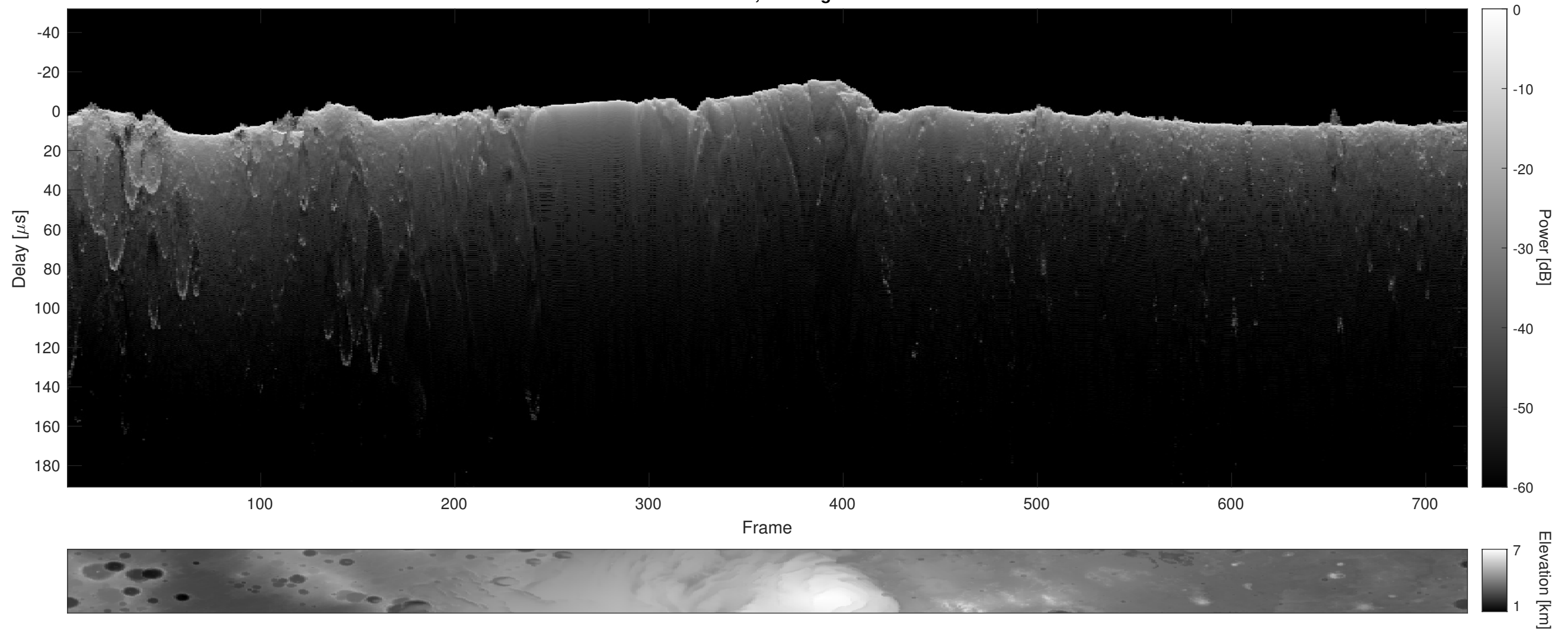
Orbit 6538, Cluttergram
