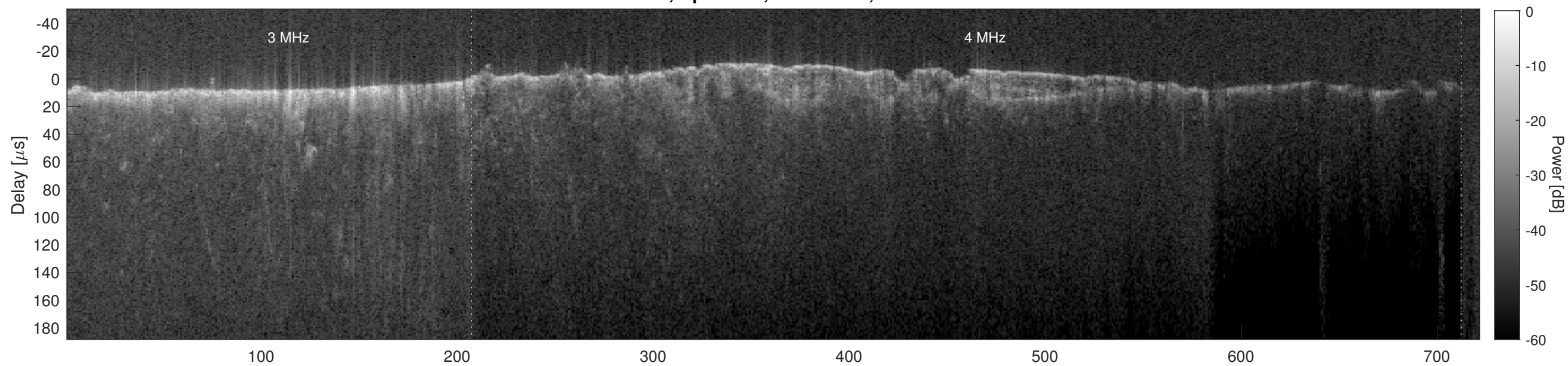
Orbit 6540, Cluttergram
