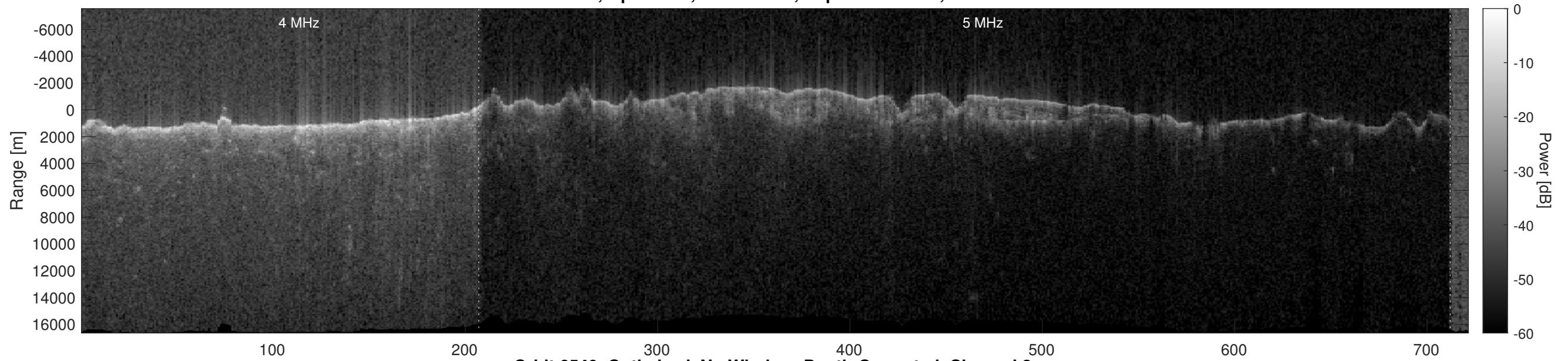
Orbit 6540, Optimized, No Window, Depth-Corrected, Channel 2
