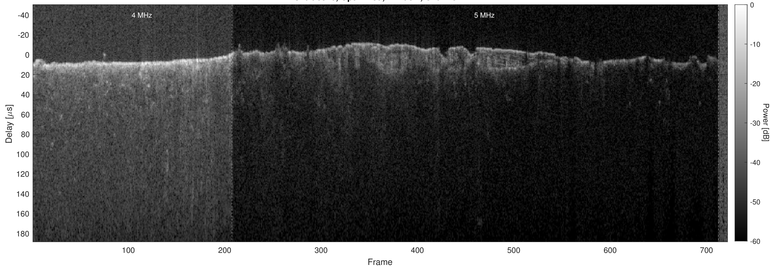
Orbit 6540, Optimized, Window, Channel 2
