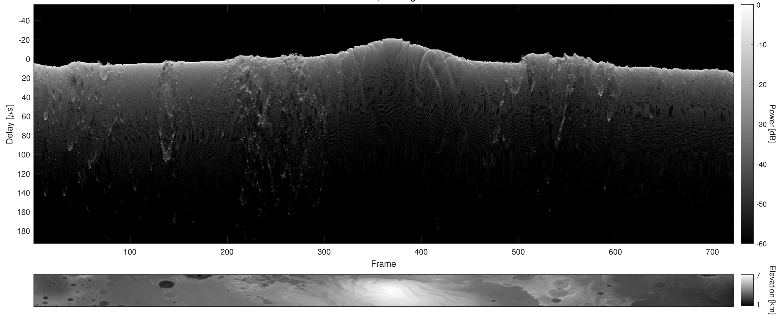
Orbit 6541, Cluttergram
