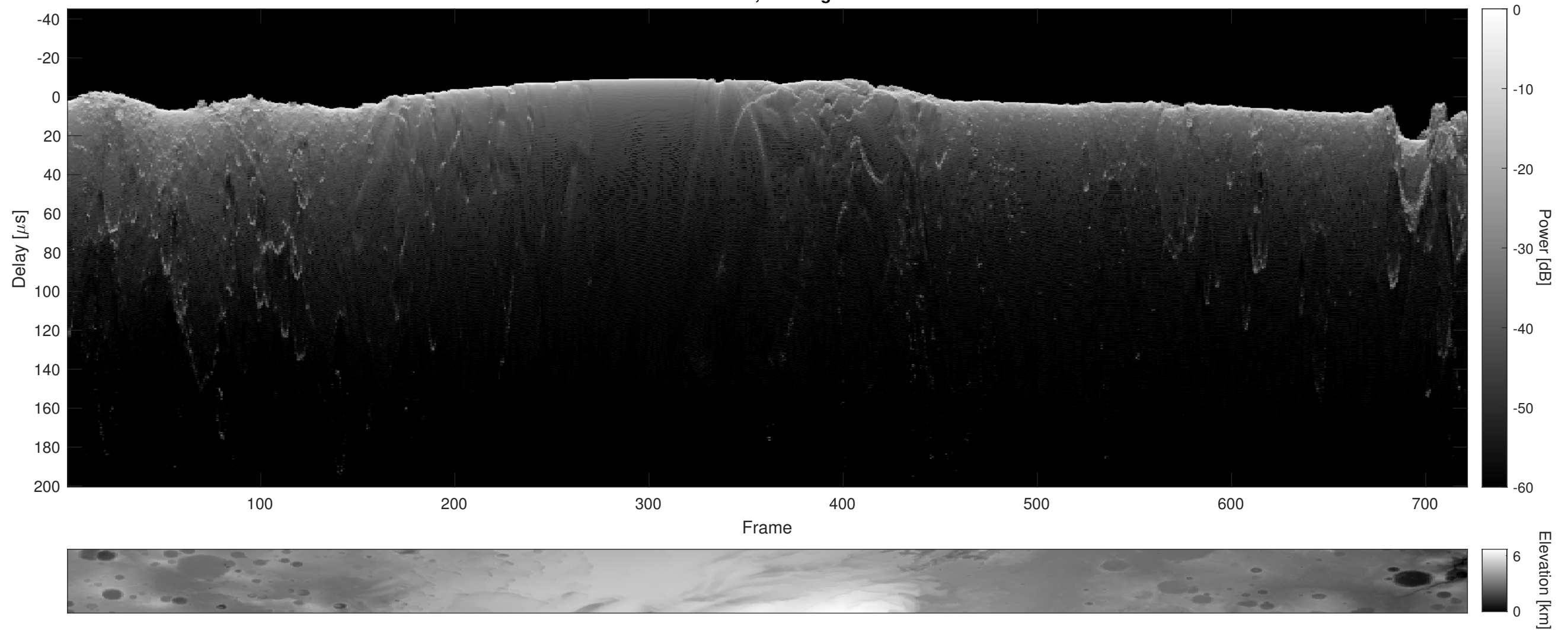
Orbit 6542, Cluttergram
