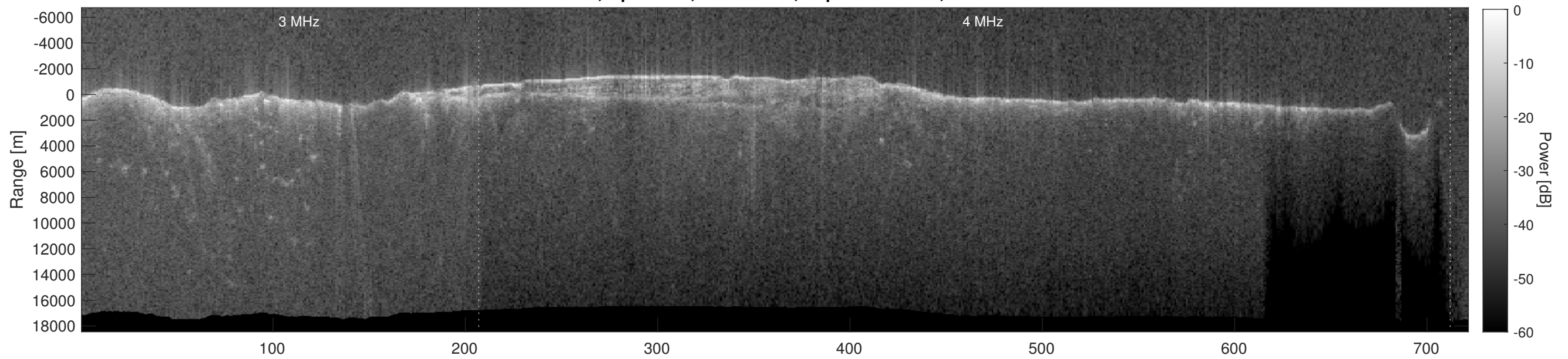
Orbit 6542, Depth-Corrected Cluttergram
