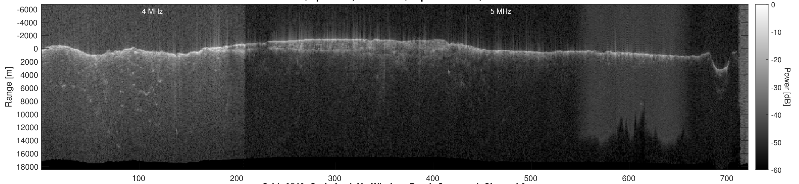
Orbit 6542, Optimized, No Window, Depth-Corrected, Channel 2
