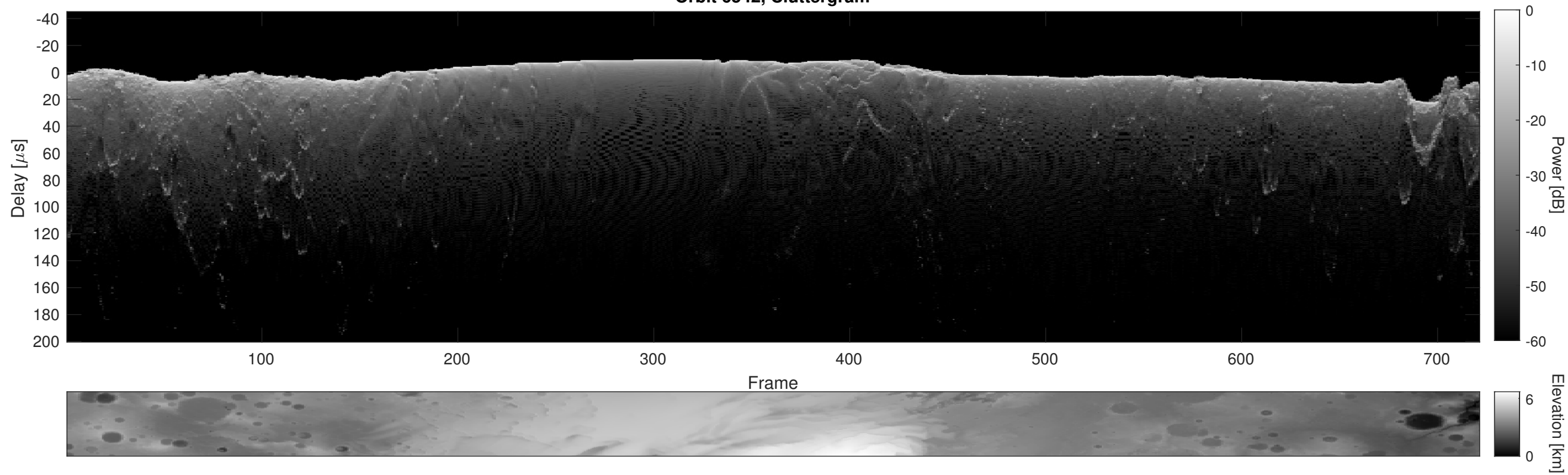
Orbit 6542, Cluttergram
