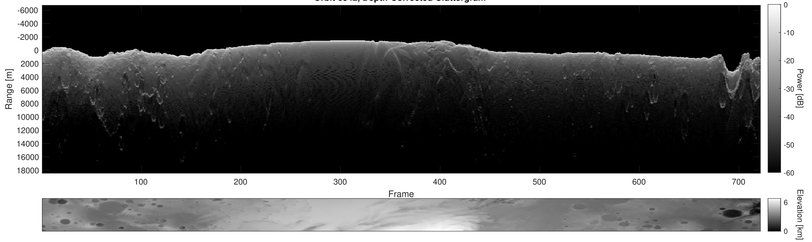
Orbit 6542, Depth-Corrected Cluttergram
