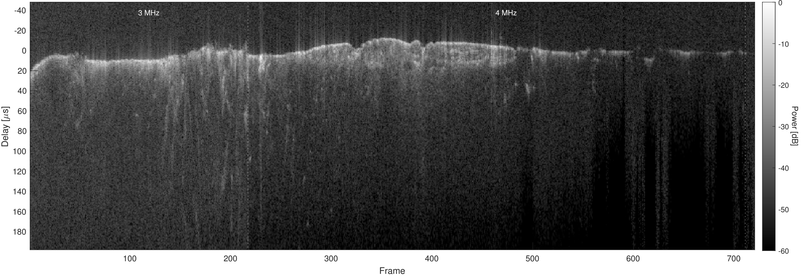
Orbit 6543, Optimized, No Window, Channel 2
