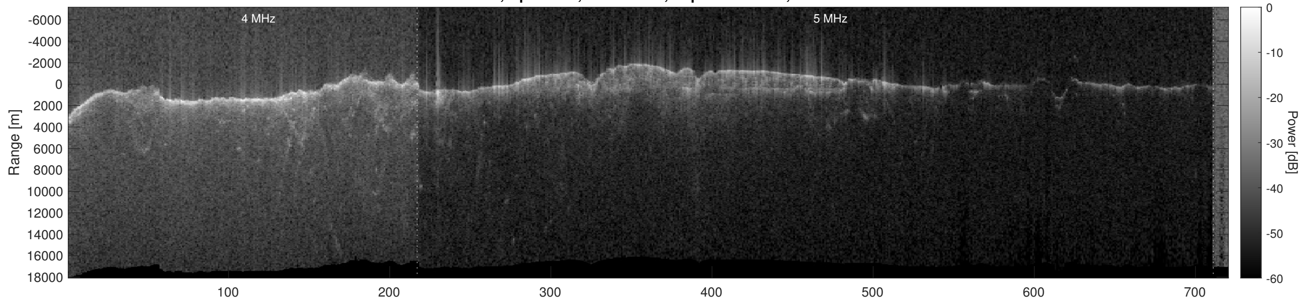
Orbit 6543, Optimized, No Window, Depth-Corrected, Channel 2
