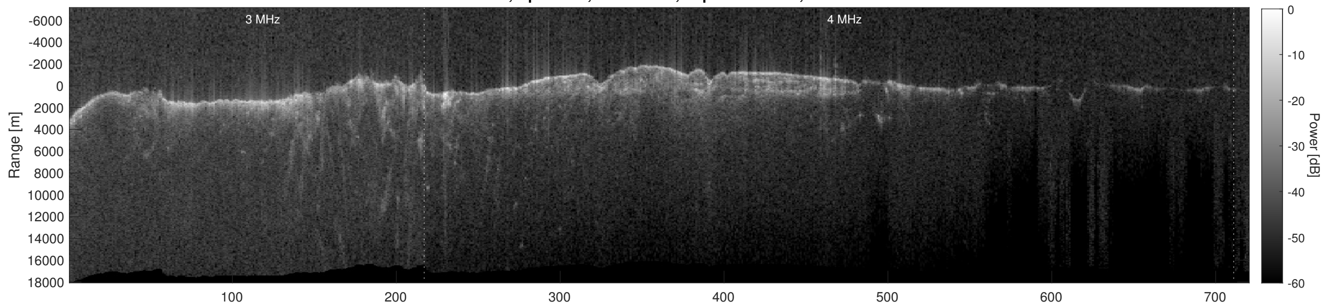
Orbit 6543, Depth-Corrected Cluttergram
