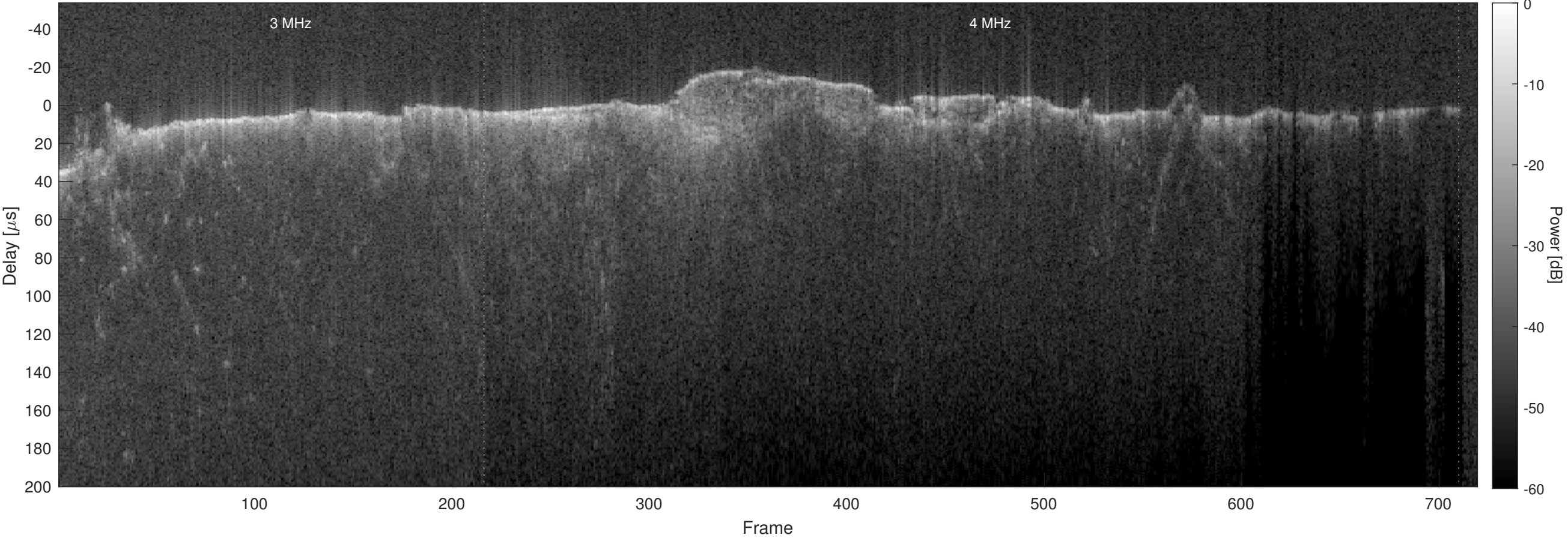
Orbit 6544, Optimized, No Window, Channel 2
