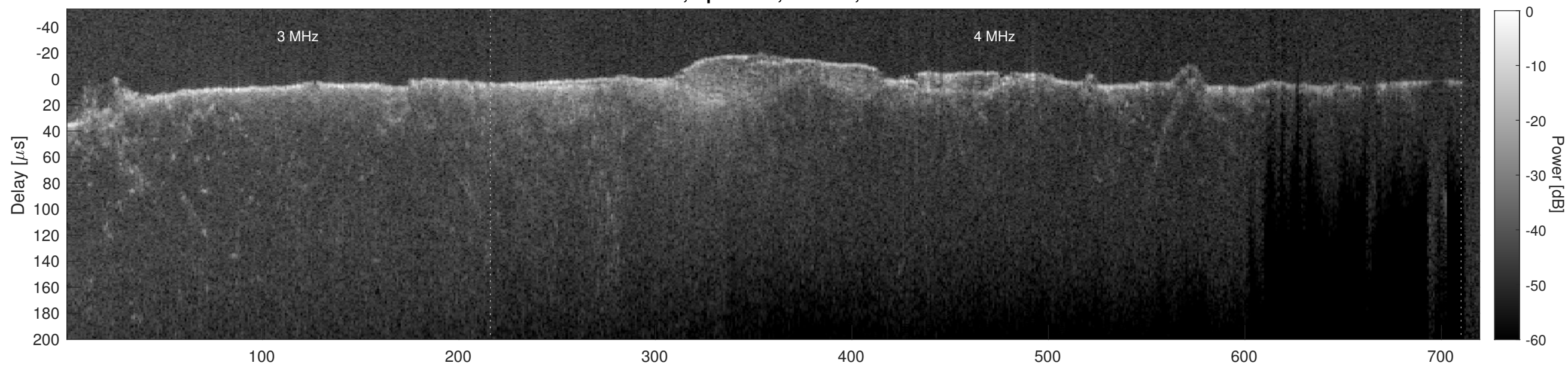
Orbit 6544, Cluttergram
