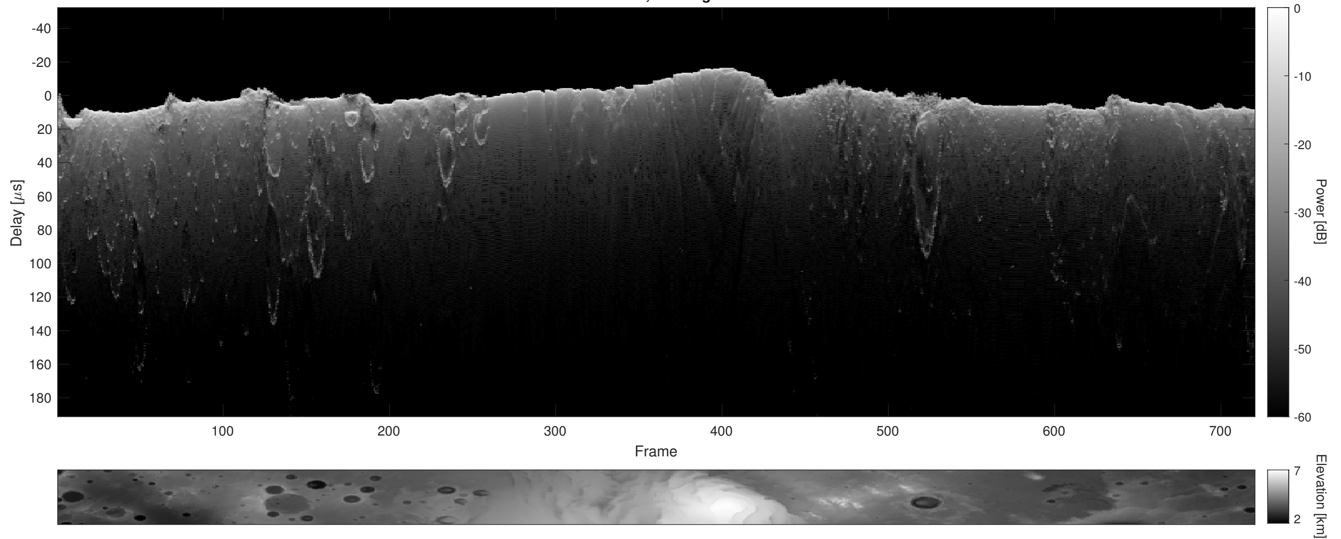
Orbit 6545, Cluttergram
