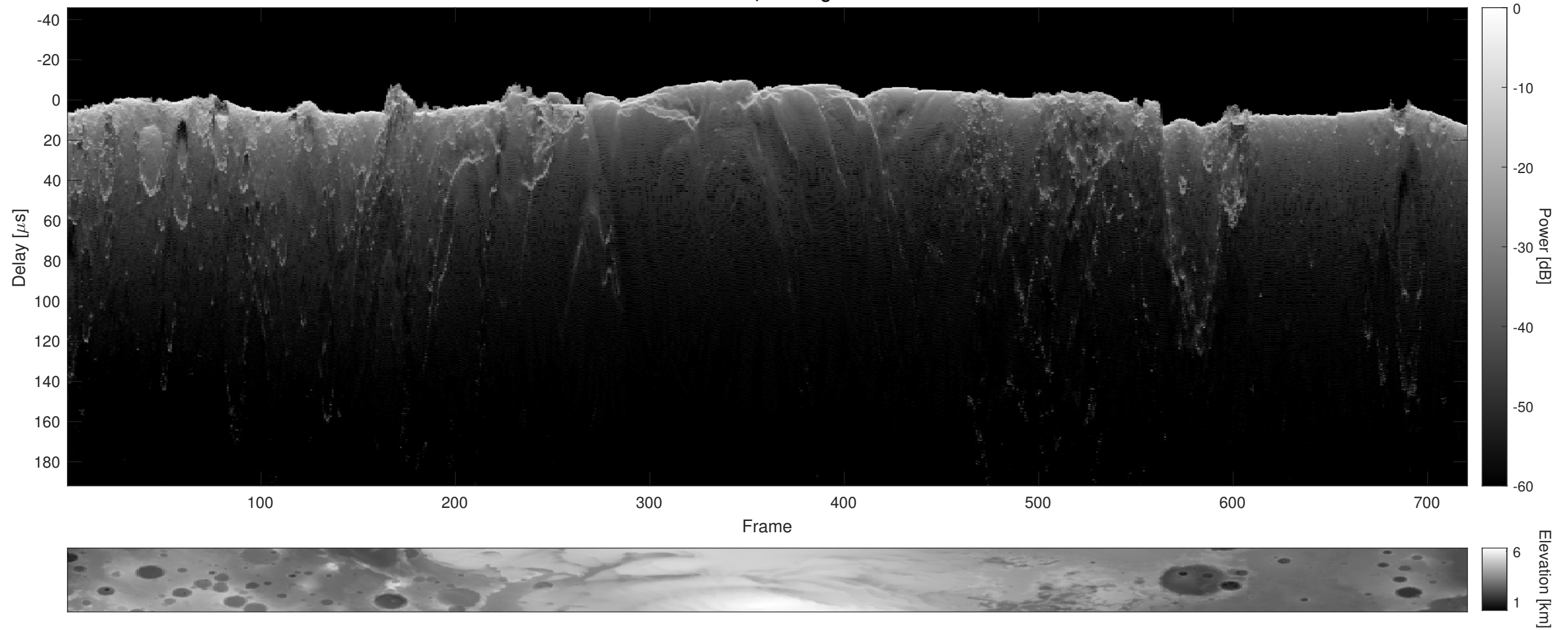
Orbit 6546, Cluttergram
